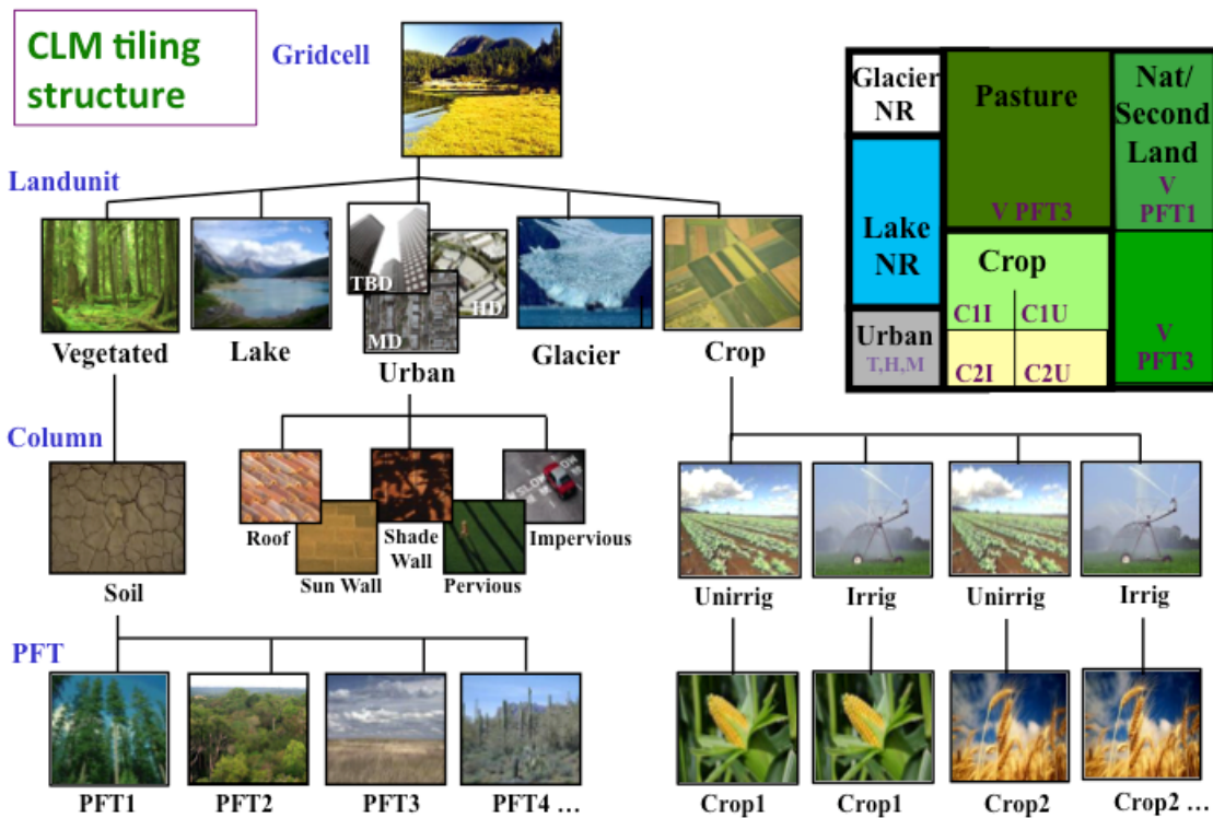
Figure #: CLM tiling structure and possible reporting under proposed subgrid structure. CLM captures a variety of ecological and hydrological sub-grid characteristics.
