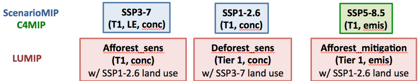
Figure 1: Example set of realistic and sensitivity studies designed to assess potential impact of strongly different land use trajectories on climate outcome.
