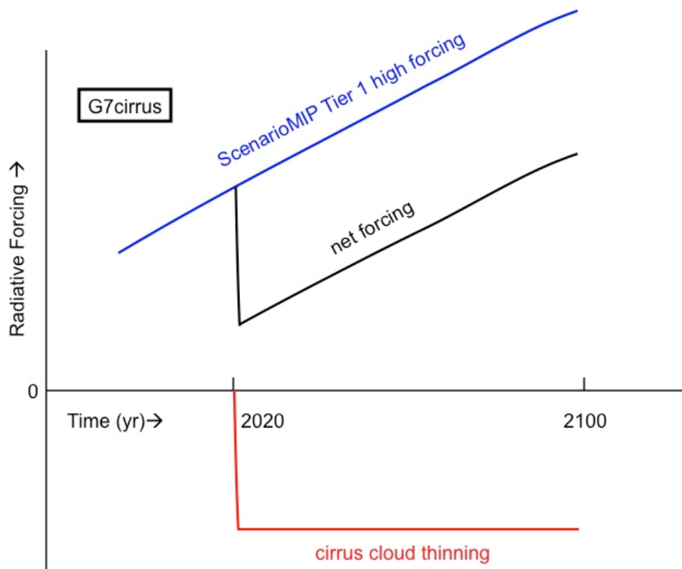
841 Figure 3. Schematic of experiment G7cirrus. Against a background scenario of the 842 ScenarioMIP Tier 1 high forcing scenario, a representation of cirrus cloud seeding 843 will reduce net forcing by a constant amount. This simulation will begin in 2020 and 844 will be conducted for 80 years.
